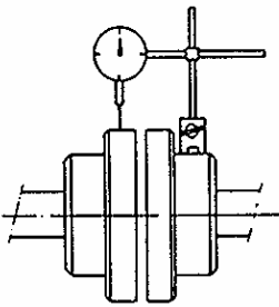
Fig. 7 – Control radial
