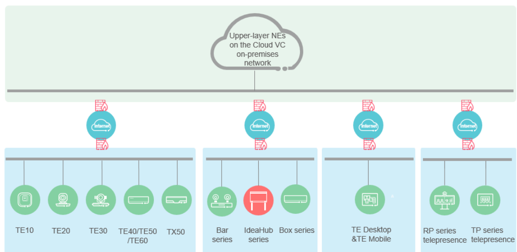
Figure 3-1 Networking scheme
